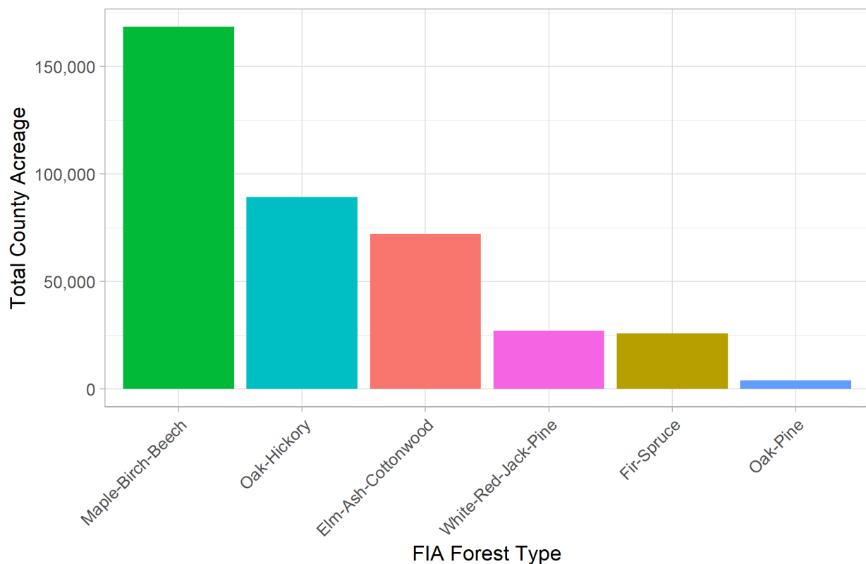
FIA Forest Type Acres in Marathon
