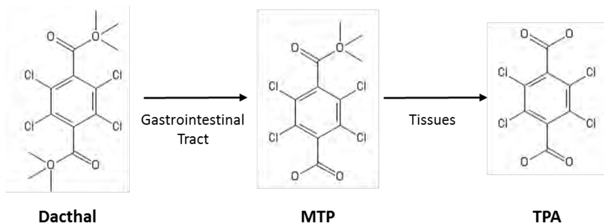
Figure A-2. Metabolism of Dacthal in the Body
