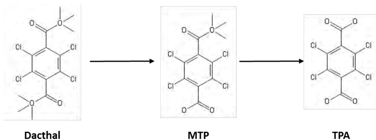
Figure A-1. Dacthal Degradation in the Environment
