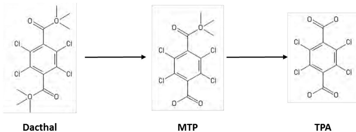
Figure A-I. Dacthal Degradation in the Environment
